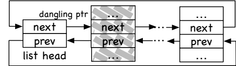
(b) Example for Error 10: the object in shadow is freed but not removed from the list.
